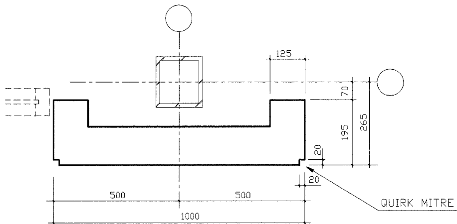
Plan Detail 3
