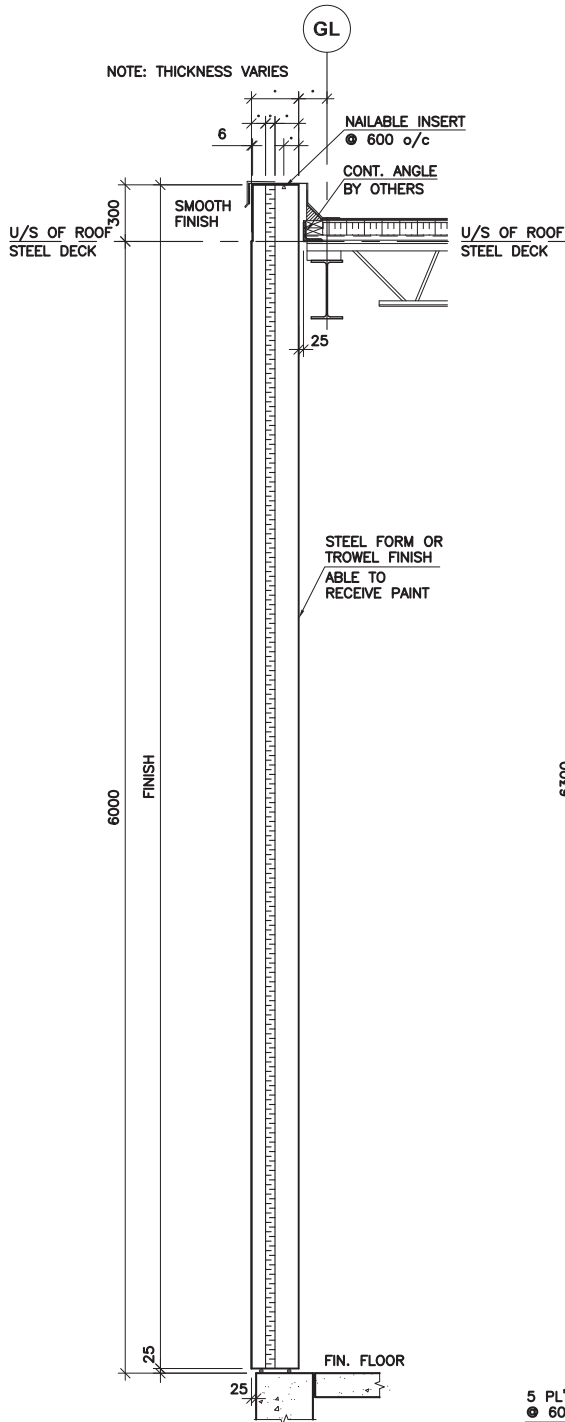
SECTION 1 FULL HEIGHT WALL
