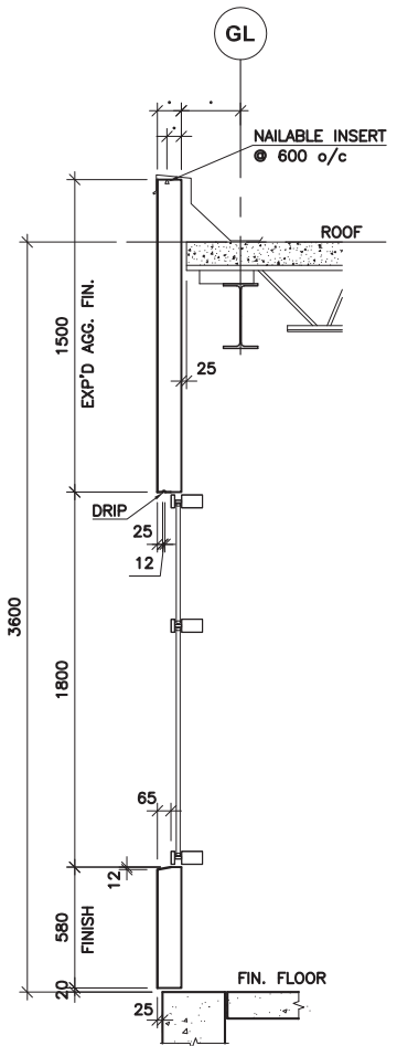
SECTION 3 OFFICE WINDOW
