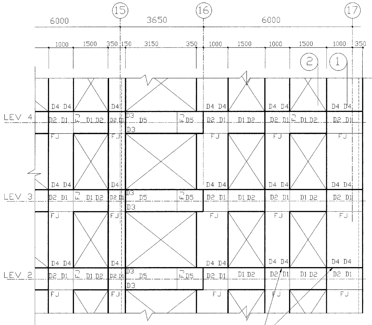
PANEL JOINTS (TYPICAL)
