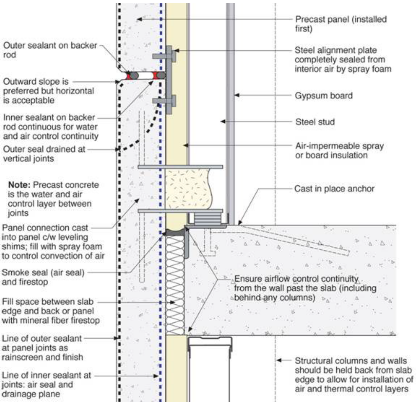
Conventional Architectural Precast Concrete Panel. Detail at horizontal joint and floor intersection demonstrating high-performance continuity of the water, air, and thermal control. Fully-drained and vented rain control at all joints.
