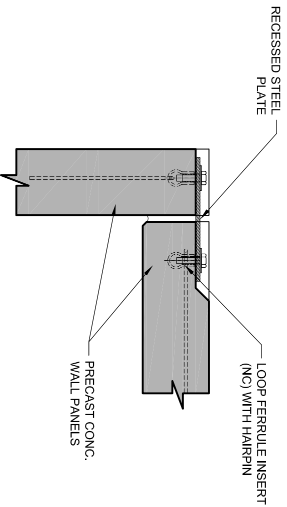
PLAN DETAIL
